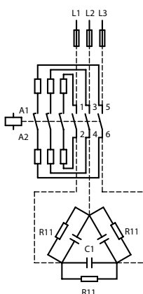
Circuit Without Quick Discharge Resistor
