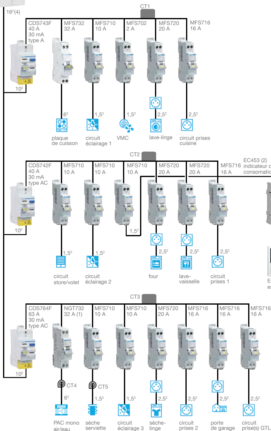
HDA260SF DB In 60 A 12 kVA individuel 500 mA type S
